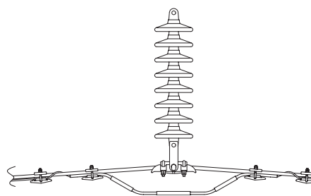
3 SUSPENSION BYPASS
