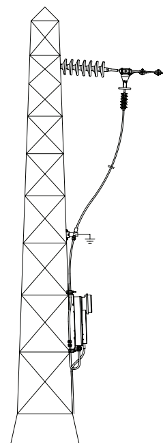
4 TERMINATION JOINT
